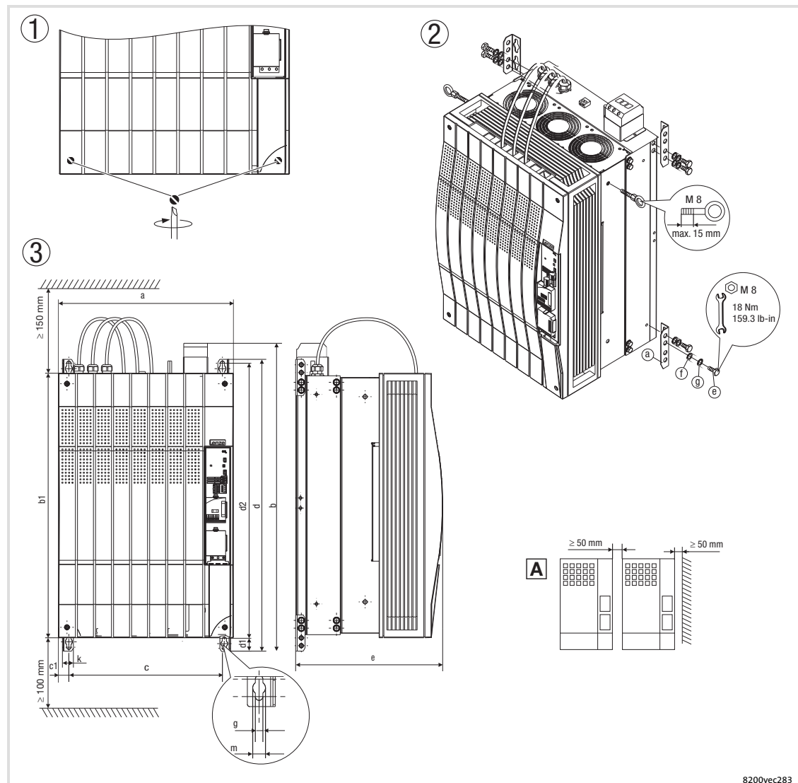
Fig. 5-31 Standard mounting with fixing brackets 75 ... 90 kW
