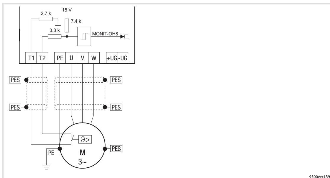
Fig. 5-11 Circuit diagram of motor connection with PTC thermistor or thermal contact (NC contact) at T1, T2
