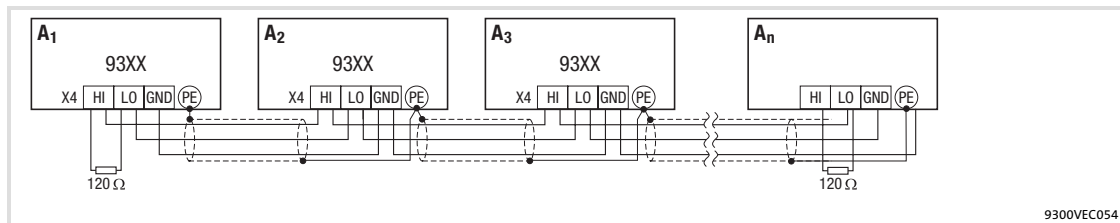
Fig. 5-14 System bus (CAN) wiring
