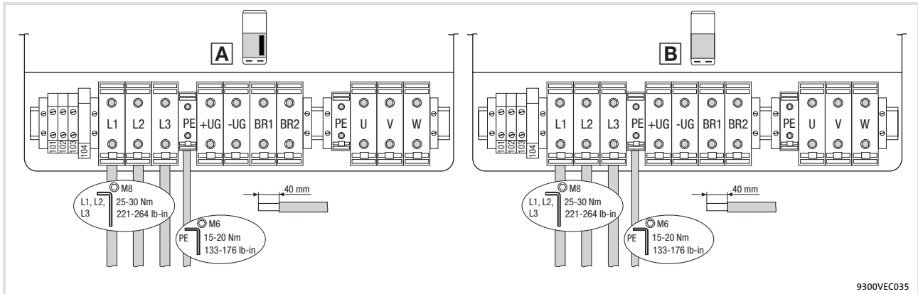
Fig. 5-8 Mains connection example
