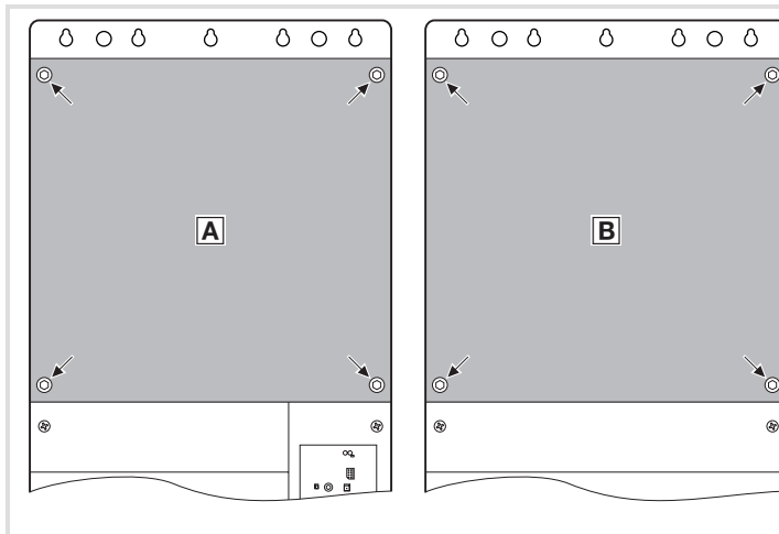
Fig. 5-6 Fastening the covers to the master and slave
