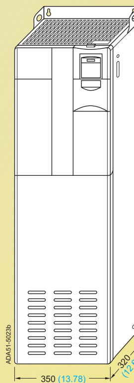
Inverter frame size F with filter
