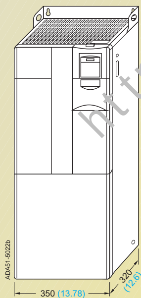
Inverter frame size F without filter
