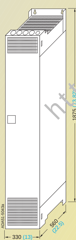
Inverter frame size GX
