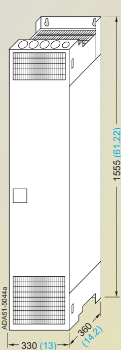
Inverter frame size FX
