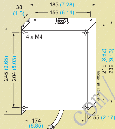
For frame size C
