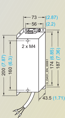
EMC filter for frame size A
