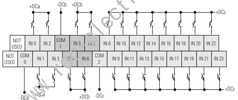
Figure 3.18 1762-L40BXB and 1762-L40BXHR Sourcing Input Wiring Diagram
