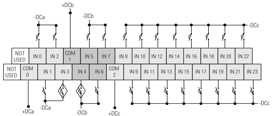
Figure 3.18 1762-L40BXB and 1762-L40BXHR Sourcing Input Wiring Diagram
