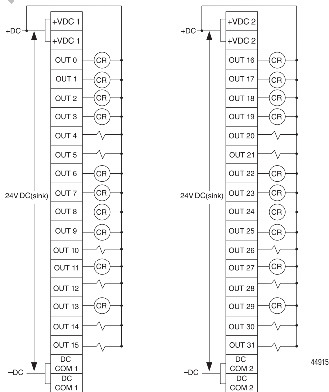
Figure 3.29 1762-0V32T Wiring Diagram
