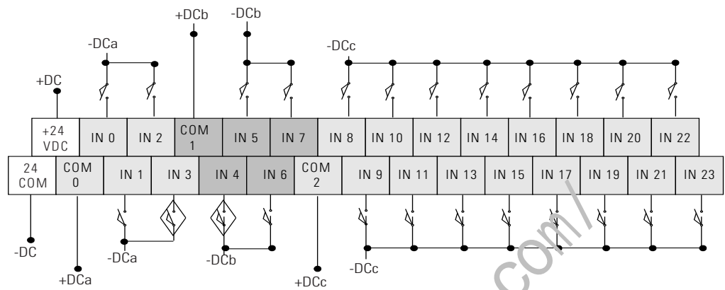
Figure 3.17 1762-L40BXB and 1762-L40BXHR Sinking Input Wiring Diagram
