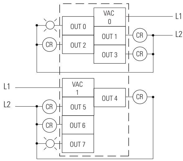
Figure 3.25 1762-OA8 Wiring Diagram
