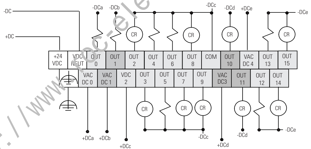
Figure 3.20 1762-L40BXB and 1762-L40BYBR Output Wiring Diagram
