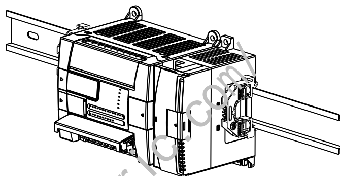
1762 Expansion I/O Connected to MicroLogix 1200 Controller
