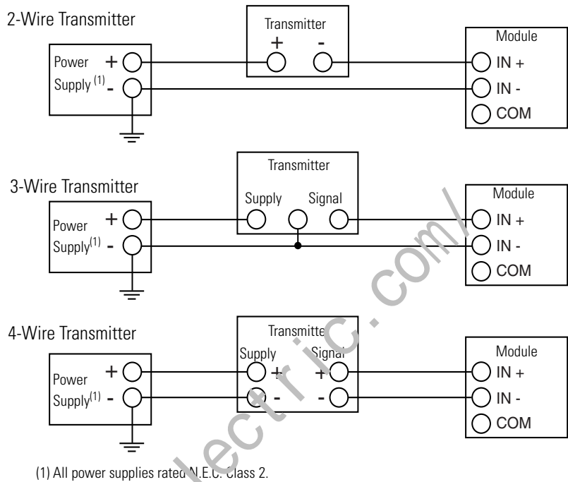
Figure 3.39 Sensor/Transmitter Types
