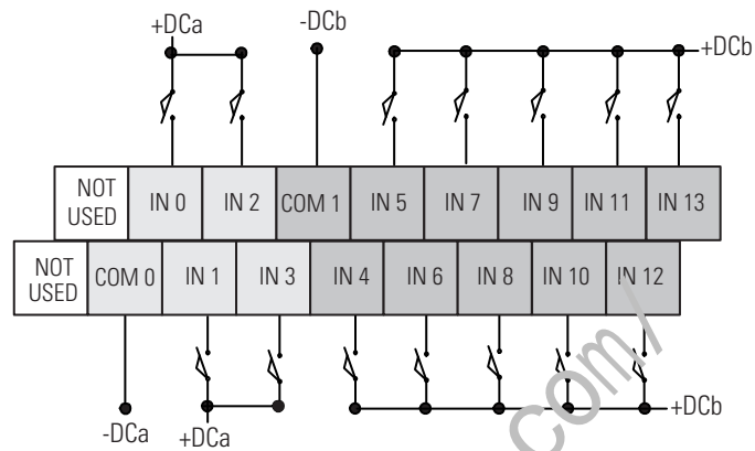
Figure 3.11 1762-L24BXB and 1762-L24BXBR Sourcing Input Wiring Diagram
