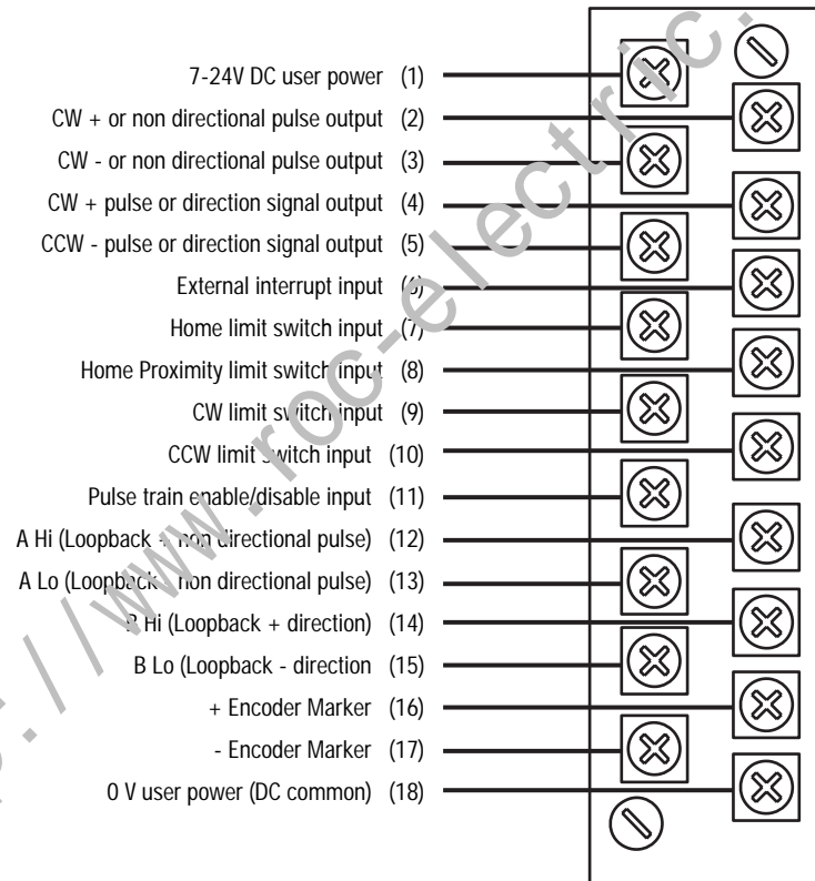
Figure 3 Input/Output Terminals
