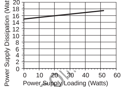
1746-P2 Power Supply Change in Power Dissipation due to Output Loading
