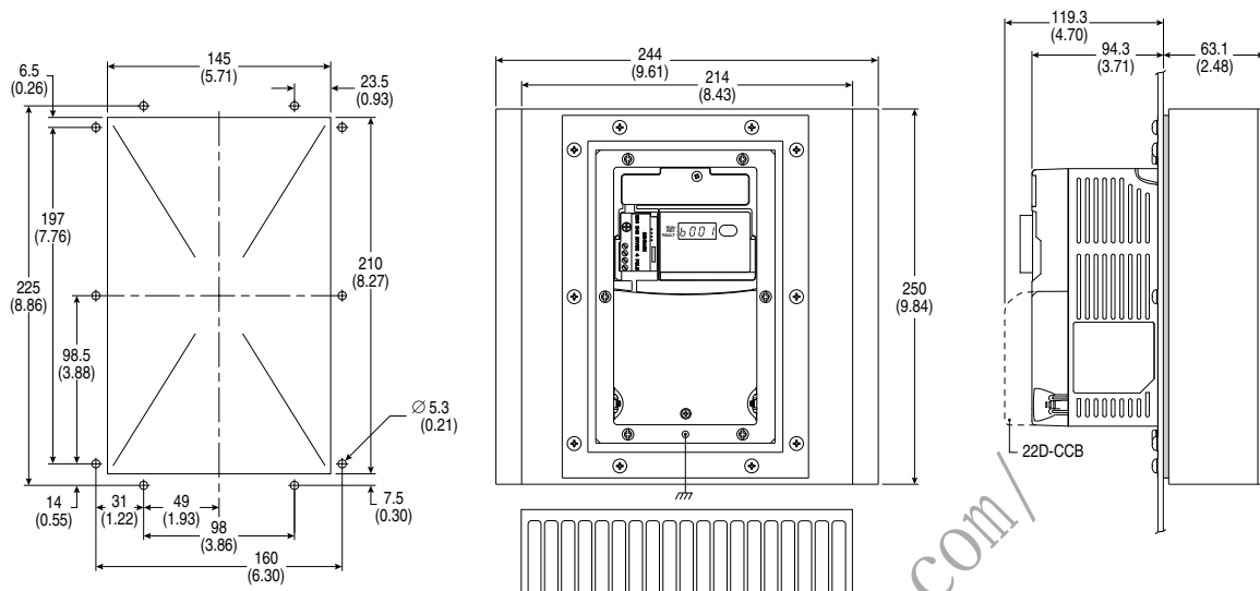
Frame B — Flange Mount
