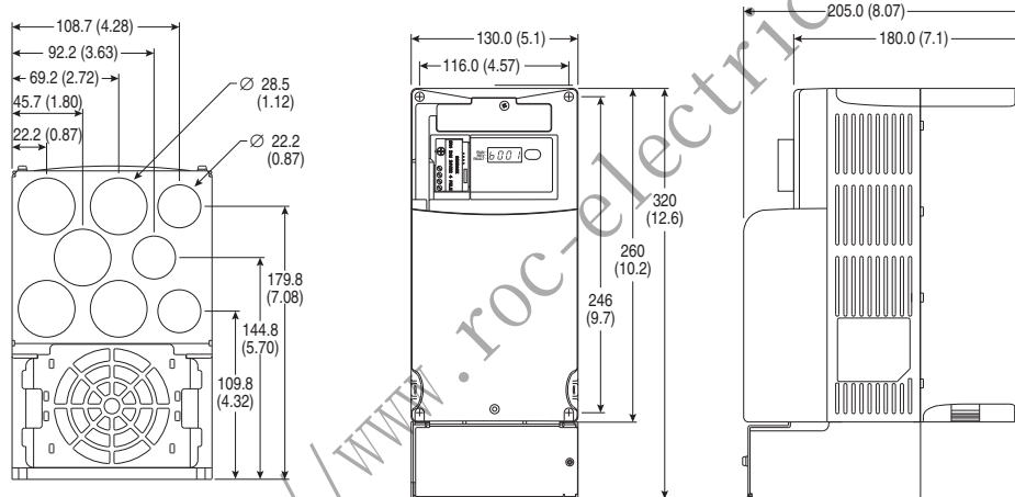
Frame C - 22-JBCC
